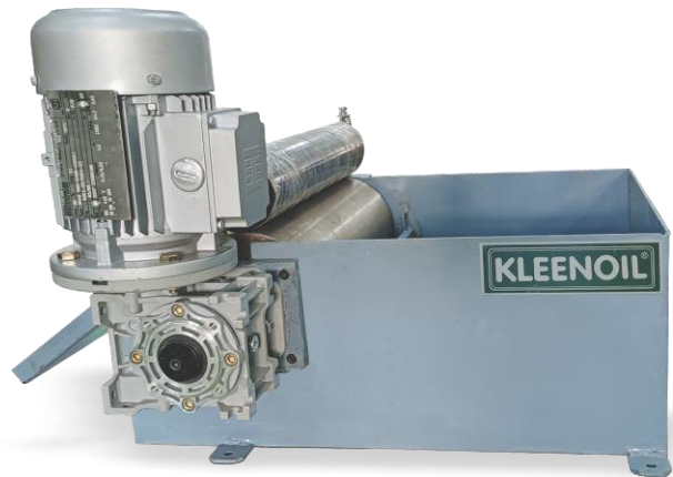
Model: MCC-100 - Suitable for Filtering: 100 LPM, Fitted with gear motor 0.25 HP, 3 Phase Magnetic Roller size: 150 x 360 MM Length, SS shell type design with Rubber Roller, scrapper etc.
